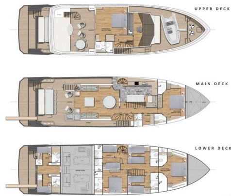
LAYOUT AEGEAN 26 M
