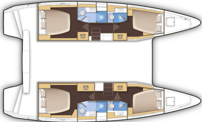
Variante 4 kabinen / 4 cabin version
